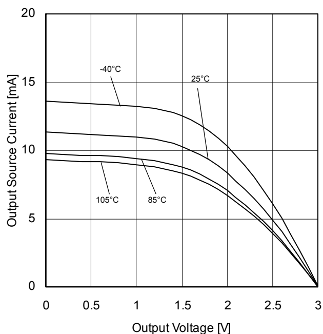
Figure 9. Output Source Current vs Output Voltage (VDD=3V)
