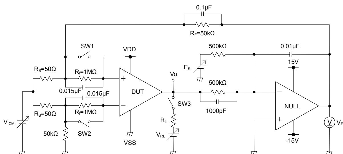
Figure 24. Test Circuit 1
