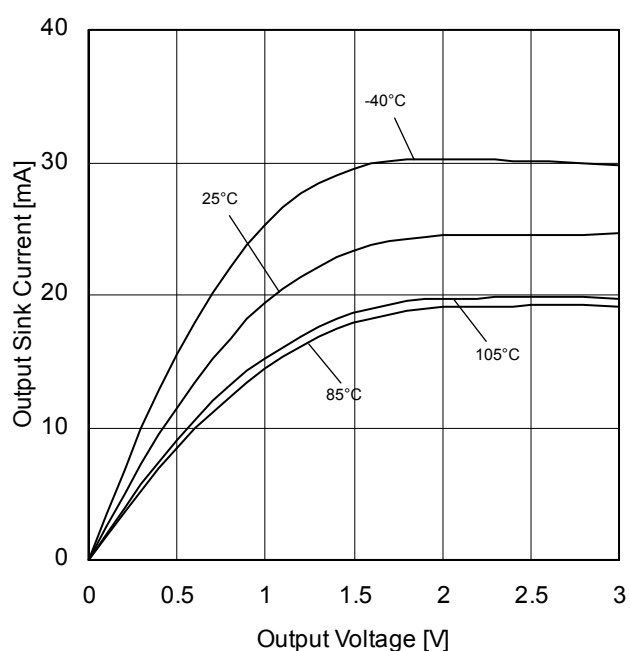
Figure 11. Output Sink Current vs Output Voltage (VDD=3V)
