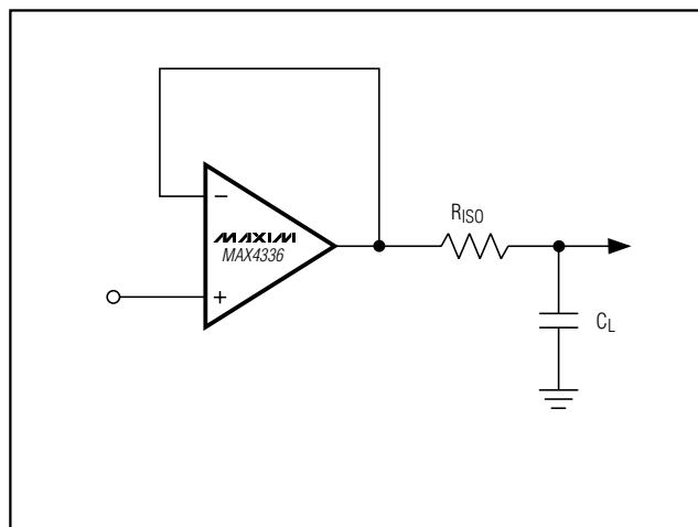
Figure 11. Capacitive-Load-Driving Circuit
