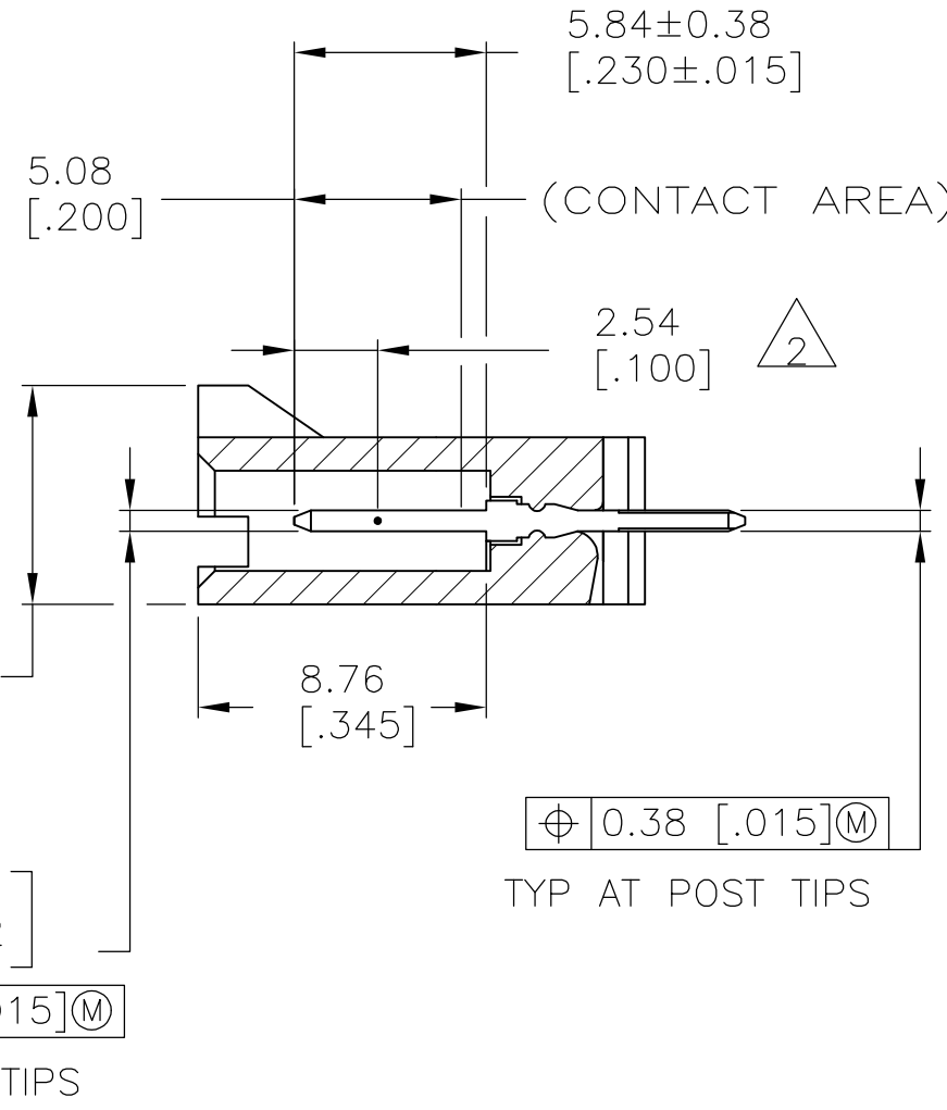
SECTION X-X
