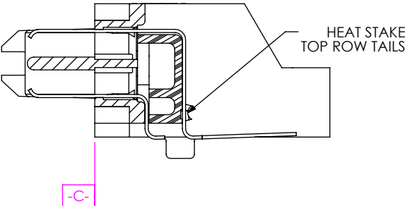
IN-PROCESS 9 (HEAT STAKE TOP ROW OF CONTACTS) (SEE INSPECTION VIEW 2 FOR ASSEMBLY ORIENTATION AND CPC'S)
