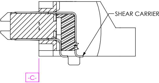
IN-PROCESS 10 (CUT OFF CARRIER) (SEE INSPECTION VIEW 2 FOR ASSEMBLY ORIENTATION AND CPC'S)
