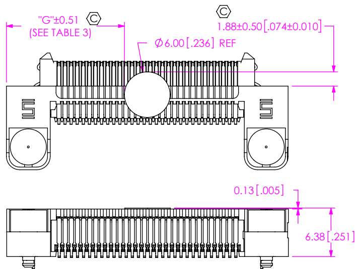
-K: PAD ERM8-030-01-X-D-RA-L-K SHOWN (USE K-DOT-.236-.343-.005)
