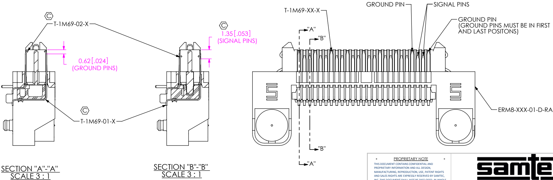
FIG 2 ERM8-025-01-X-D-RA-DS-L SHOWN (DIFFERENT AS SHOWN, OTHERWISE SAME AS FIG 1)
