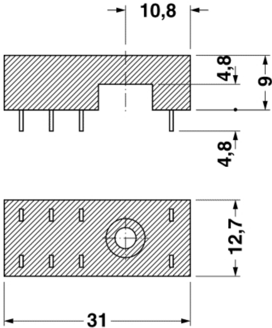
Dimensional drawing
