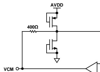
Figure 42. Equivalent VCM Circuit
