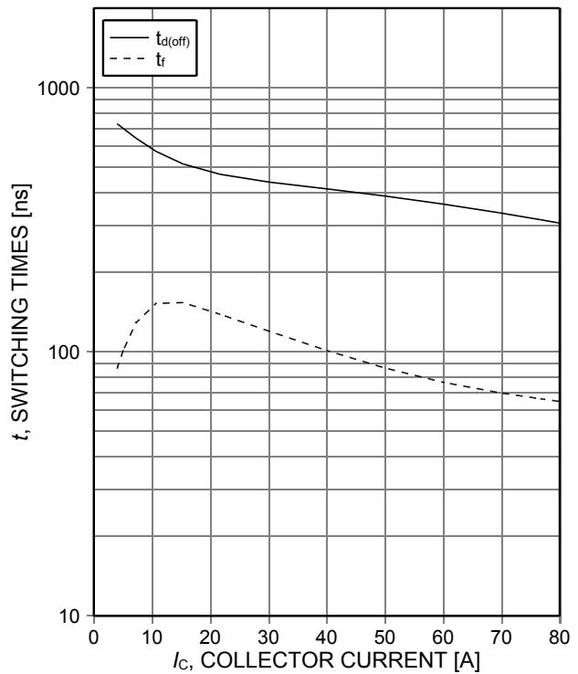
Figure 8. Typical switching times as a function of collector current (inductive load, T_j=175^\circ\text{C} , V_{CE}=600\text{V} , V_{GE}=0/15\text{V} , R_{G(on)}=7.5\Omega , R_{G(off)}=7.5\Omega , dynamic test circuit in Figure E)
