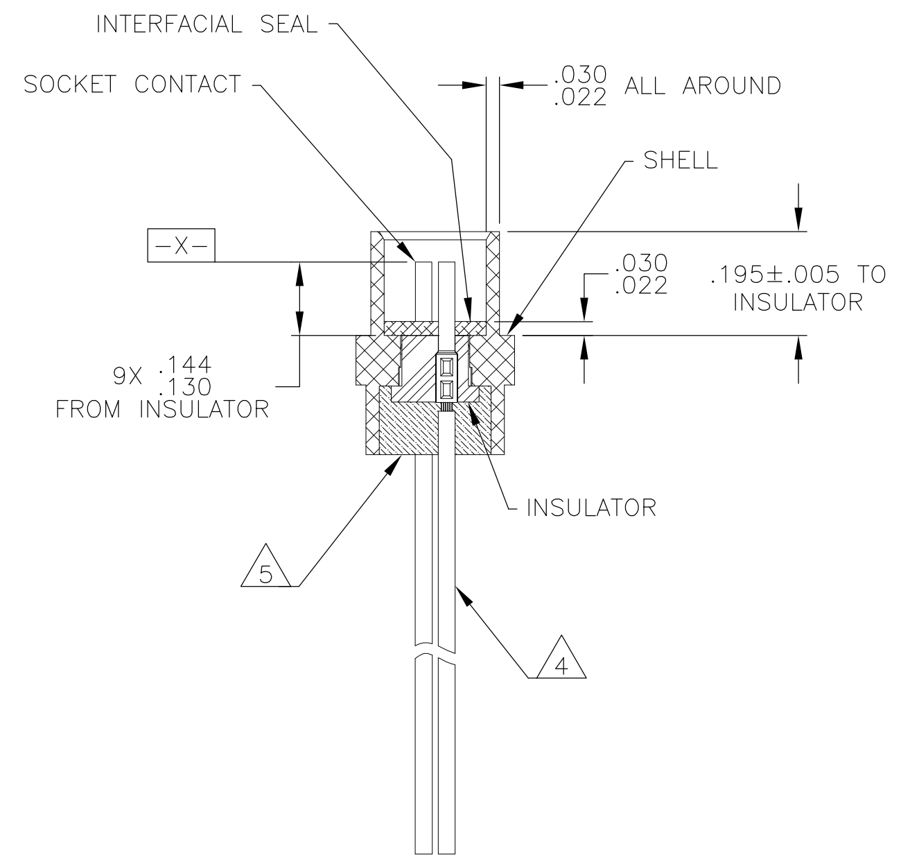
VIEW B-B
