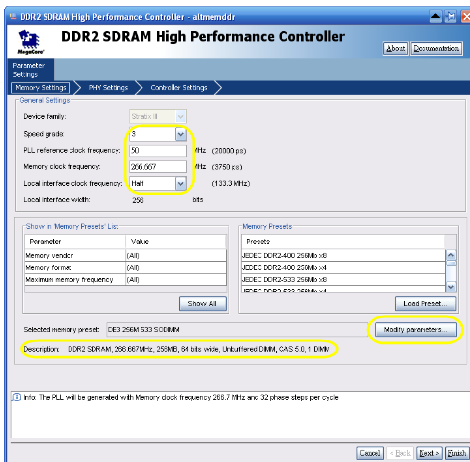
Figure 5.119. Memory Settings in DDR2 Controller
