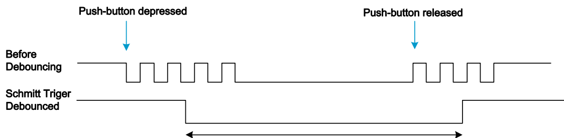
Figure 2.7. Switch debouncing
