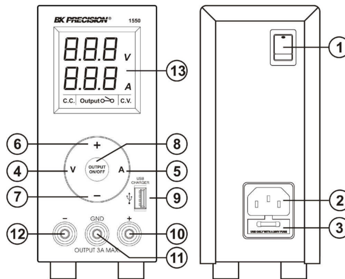
Figure 2.1: Front Panel
