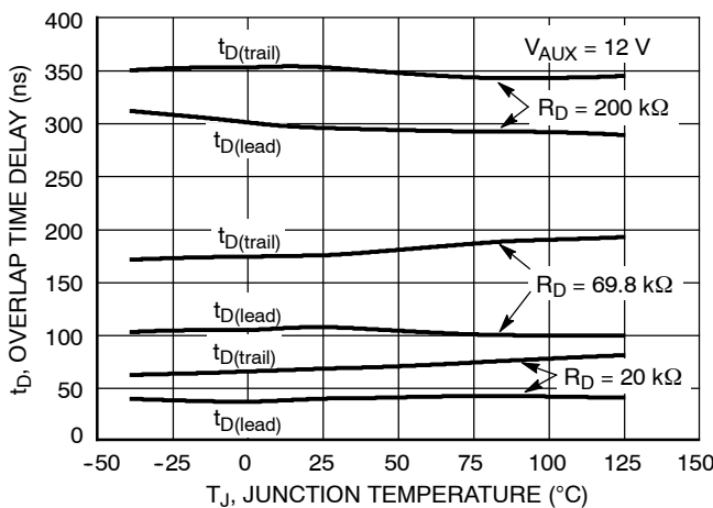
Figure 29. Overlap Time Delay vs. Junction Temperature
