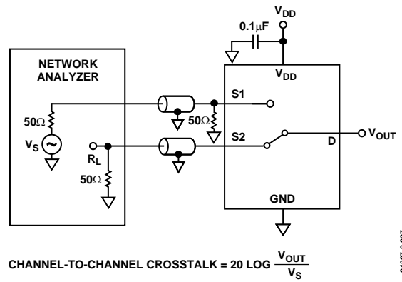
Figure 27. Channel-to-Channel Crosstalk
