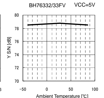
Fig.96 SN_{\gamma} vs. Ambient Temperature
