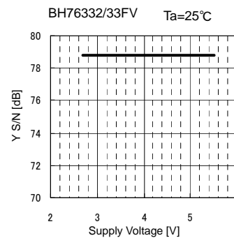
Fig.95 SN_{\gamma} vs. Supply Voltage
