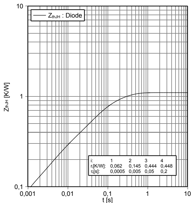
Transienter Wärmewiderstand Diode, D5-D6 transient thermal impedance Diode, D5-D6
