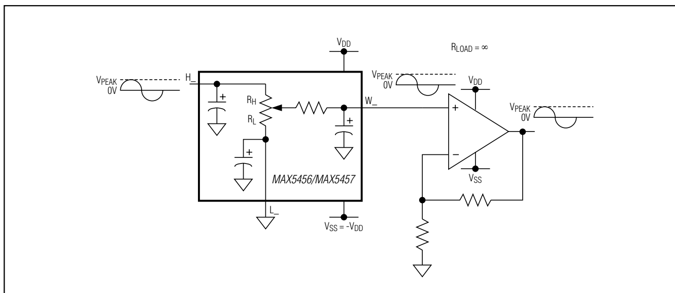
Typical Application Circuit (Dual Supplies)
