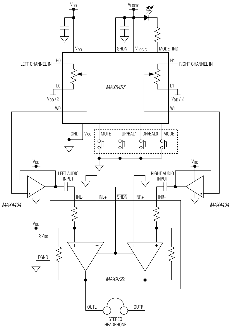
Figure 6. Volume/Balance Control
