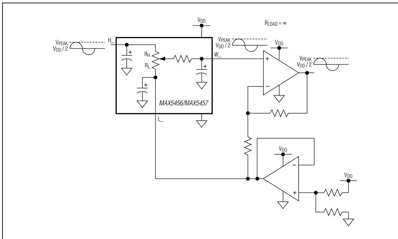
Typical Application Circuit (Single Supply)
