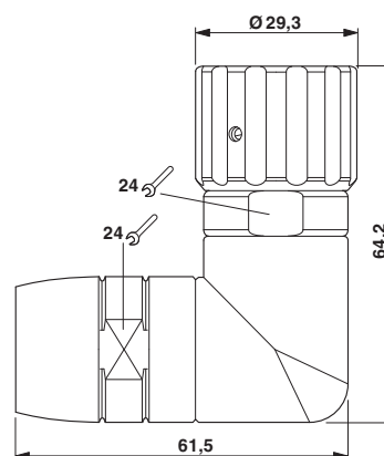
Dimensional drawing
