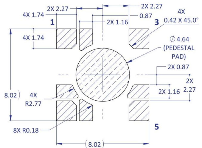
Figure 2a: Recommended solder pad layout for anode, cathode, and thermal pad for non-pedestal and pedestal design
