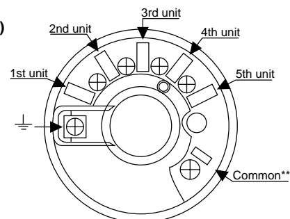
Cabling (base viewed from above)
