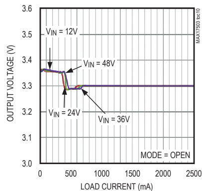
MAX17503, 3.3V OUTPUT, PFM MODE, FIGURE 4b CIRCUIT LOAD AND LINE REGULATION
