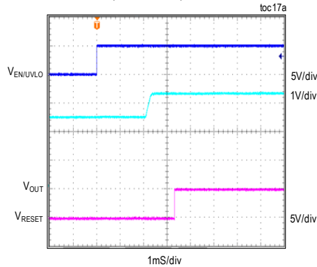
MAX17503S, SOFT-START WITH 2.5V PREBIAS, 3.3V OUTPUT, PFM MODE, FIGURE 4d CIRCUIT
