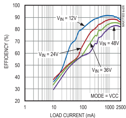
MAX17503, 3.3V OUTPUT, DCM MODE, FIGURE 4b CIRCUIT EFFICIENCY vs. LOAD CURRENT
