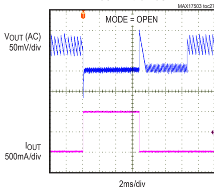
MAX17503 3.3V OUTPUT, PFM MODE (LOAD CURRENT STEPPED FROM 5mA TO 1A), FIGURE 4b CIRCUIT
