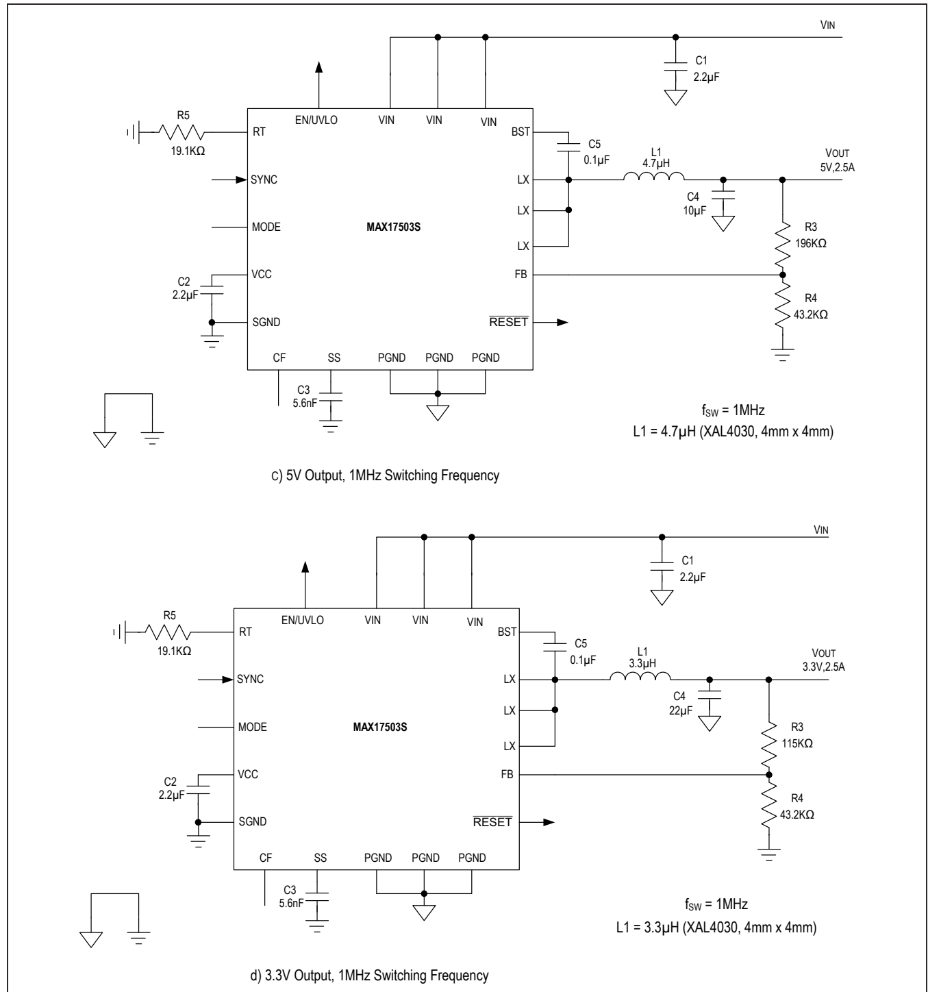
Figure 4. MAX17503/MAX17503S Typical Application Circuits (continued)
