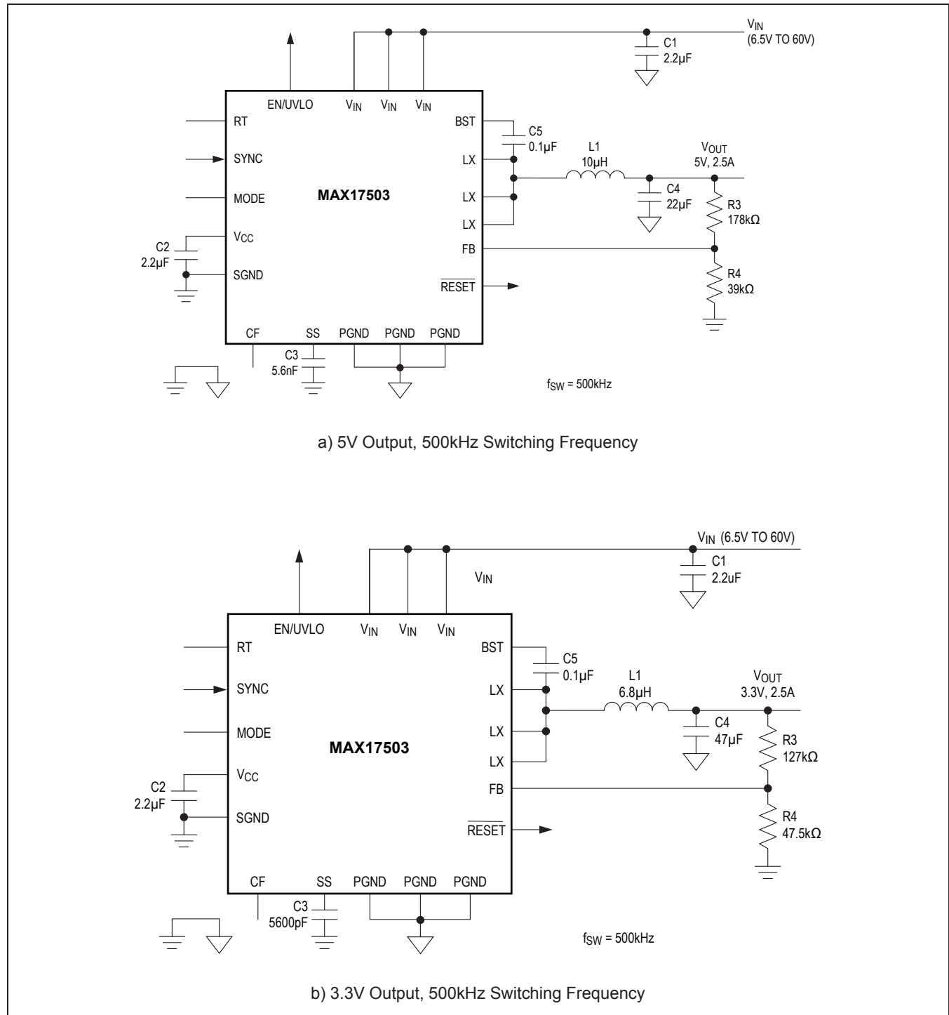
Figure 4. MAX17503/MAX17503S Typical Application Circuits
