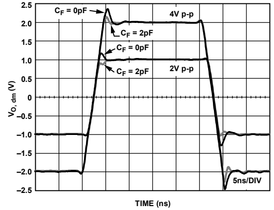
Figure 34. Large Signal Transient Response for Various C_f
