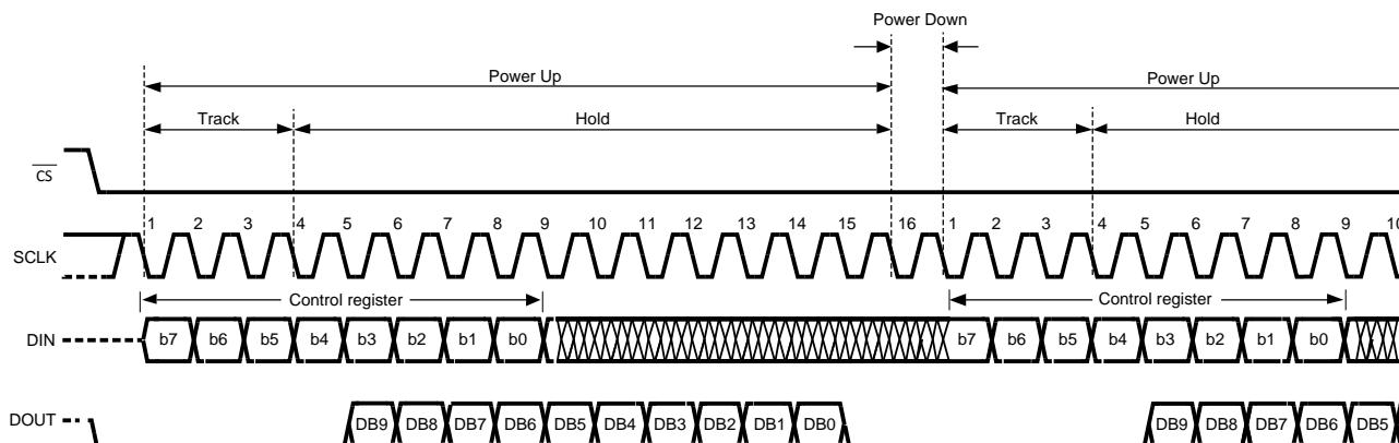
Figure 2. ADC102S051 Operational Timing Diagram
