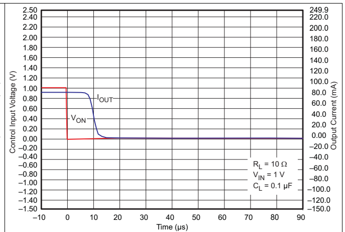
Figure 49. t_{OFF} Response
