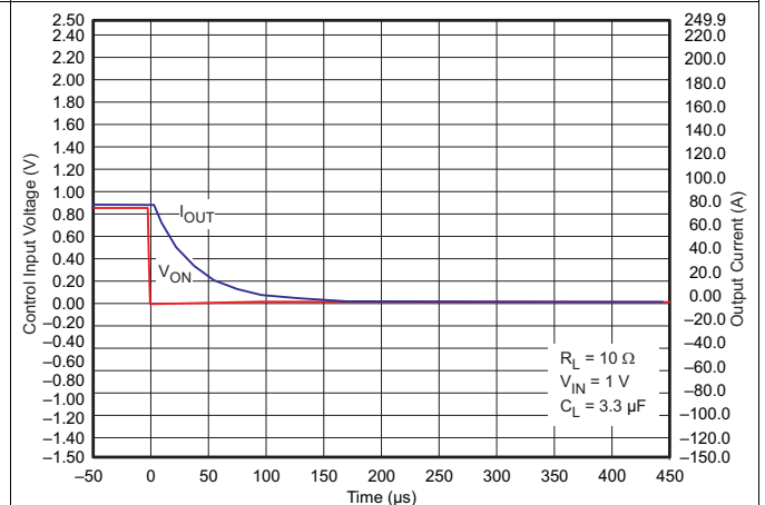
Figure 51. t_{OFF} Response
