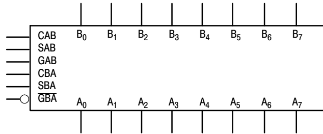
Figure 6. Logic Symbol
