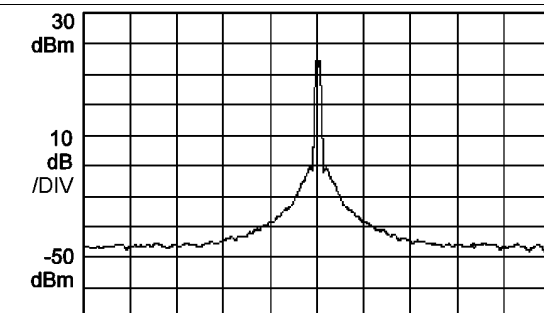
Figure 2. Transmit Spectrum
