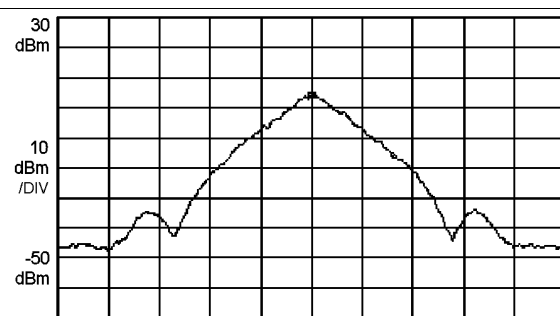
Figure 2. Transmit Spectrum
