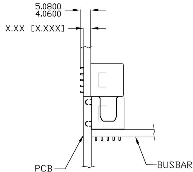
MATED CONDITION
