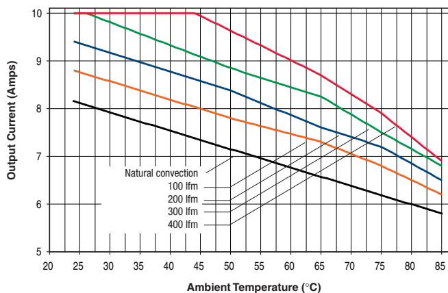
UVQ-12/10-D48N: Maximum Current Temperature Derating (No baseplate, V_{IN} = 48V , transverse air flow)
