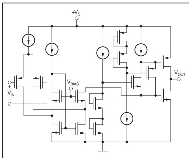
Figure 1. OPA30x Classic Two-Stage Topology
