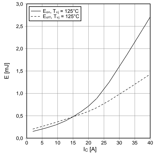
Schaltverluste IGBT-Wechselr. (typisch) switching losses IGBT-inverter (typical) E_{on} = f(I_C) , E_{off} = f(I_C) V_{GE} = \pm 15\text{ V} , R_{Gon} = 47\ \Omega , R_{Goff} = 47\ \Omega , V_{CE} = 300\text{ V}
