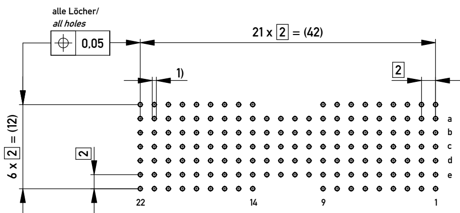
board hole pattern (component mounting side)
