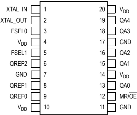
Figure 2. MPC9817 20-Lead SSOP Package Pinout (Top View)
