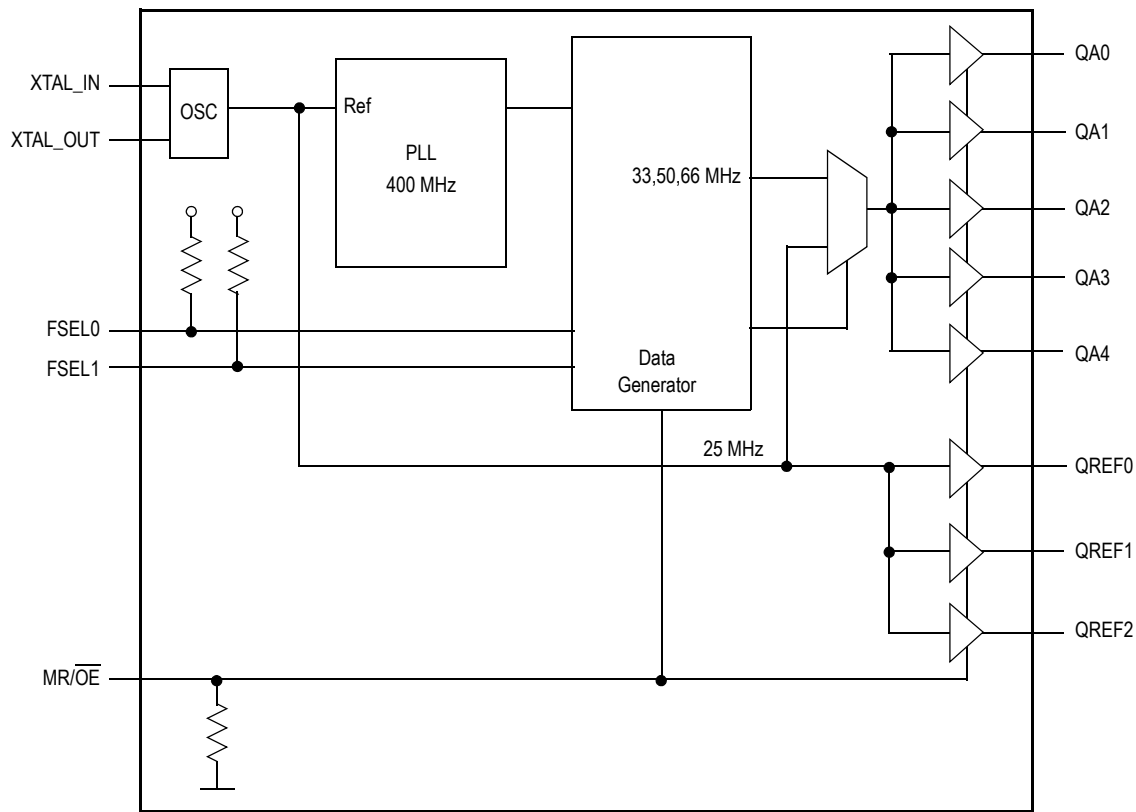
Figure 1. MPC9817 Logic Diagram
