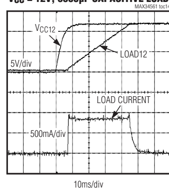
TURN-ON WAVEFORMS V_{CC} = 12\text{V} , 3300\mu\text{F} CAPACITIVE LOAD
