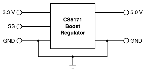
Figure 2. Application Diagram
