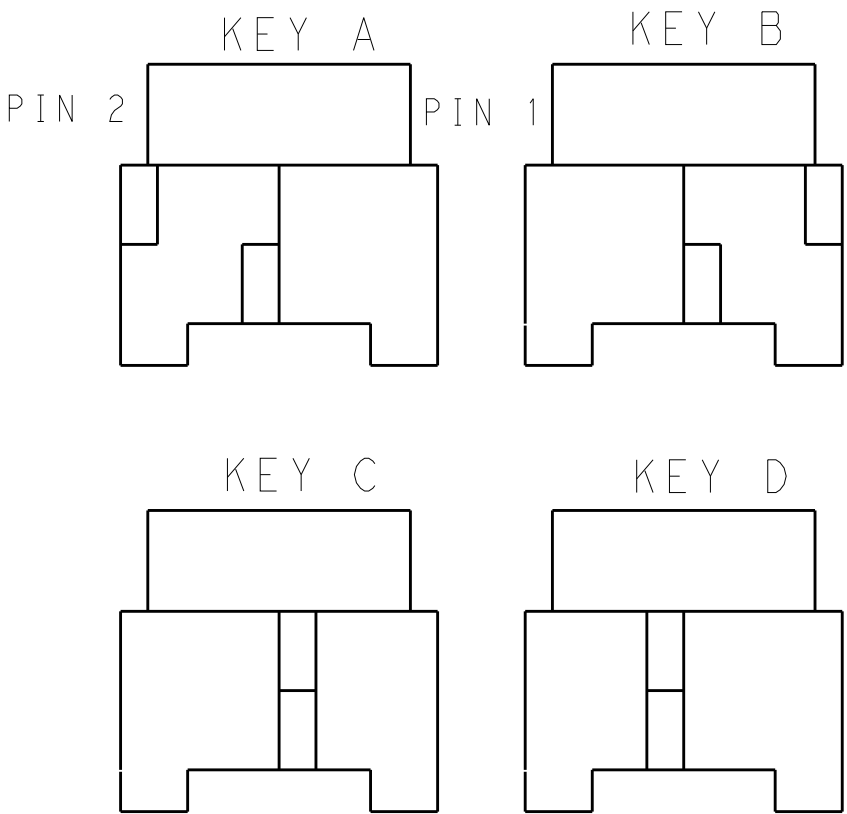
1*2 POSITIONS
