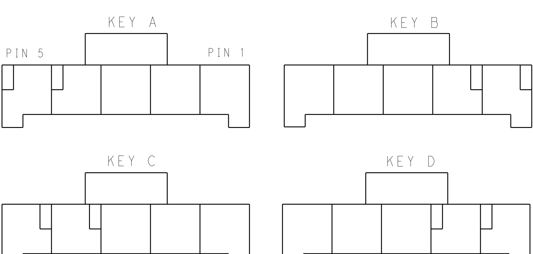
1*5 POSITIONS
