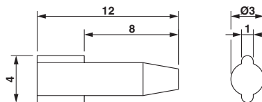
Dimensional drawing
