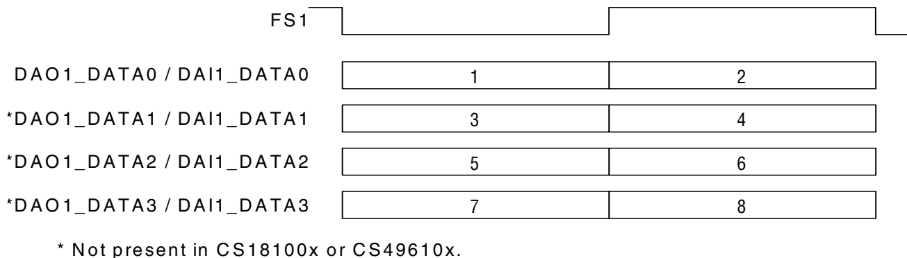
Figure 4. Channel Structure for Synchronous Serial Audio at 64FS (One Sample Period) - CS18100x/CS49610x & CS18101x/CS49611x
