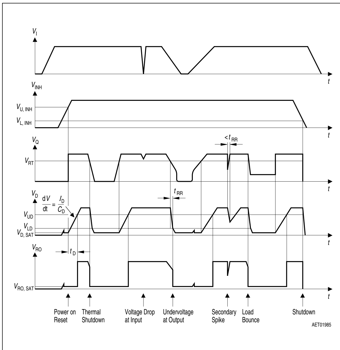
Figure 5 Time Response
