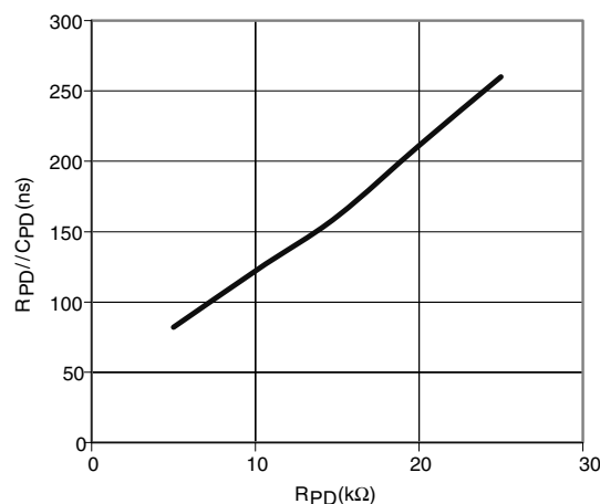
Powerdown Timeout vs. R_{PD}
