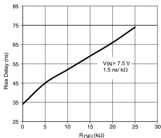
Rise Delay vs. R_{DEL}
