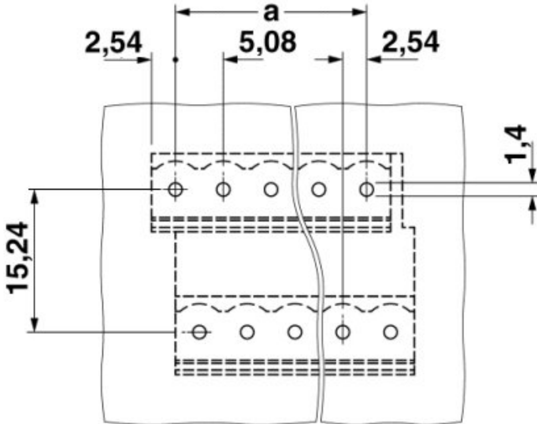
Drilling diagram
