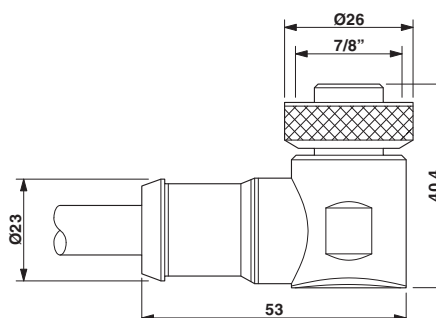
Dimensional drawing
