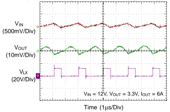
Voltage Ripple
