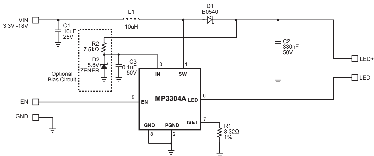
Figure 6 — Driving 27 WLEDs (9 WLEDs in Series and 3 Strings Paralleled) with 3.3V-18V Input Voltage
