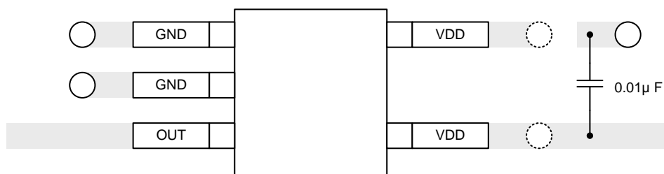
Figure 19. SC70 Package Recommended Layout
