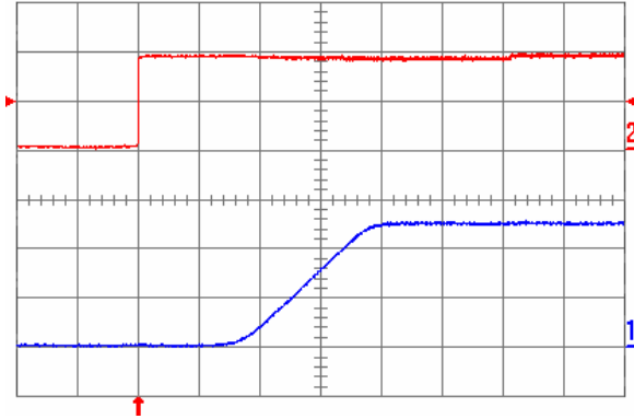
Fig. 2.5V.5: Turn-on transient for V_{out} = 2.5\text{ V} with the application of Enable signal at full rated load current (resistive) and 100\text{ }\mu\text{F} external capacitance at V_{in} = 5\text{ V} . Top trace: Enable signal (2 V/div.); Bottom trace: output voltage (1 V/div.); Time scale: 2 ms/div.
