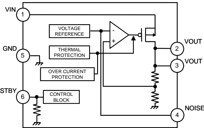
Figure 2. Block diagram
