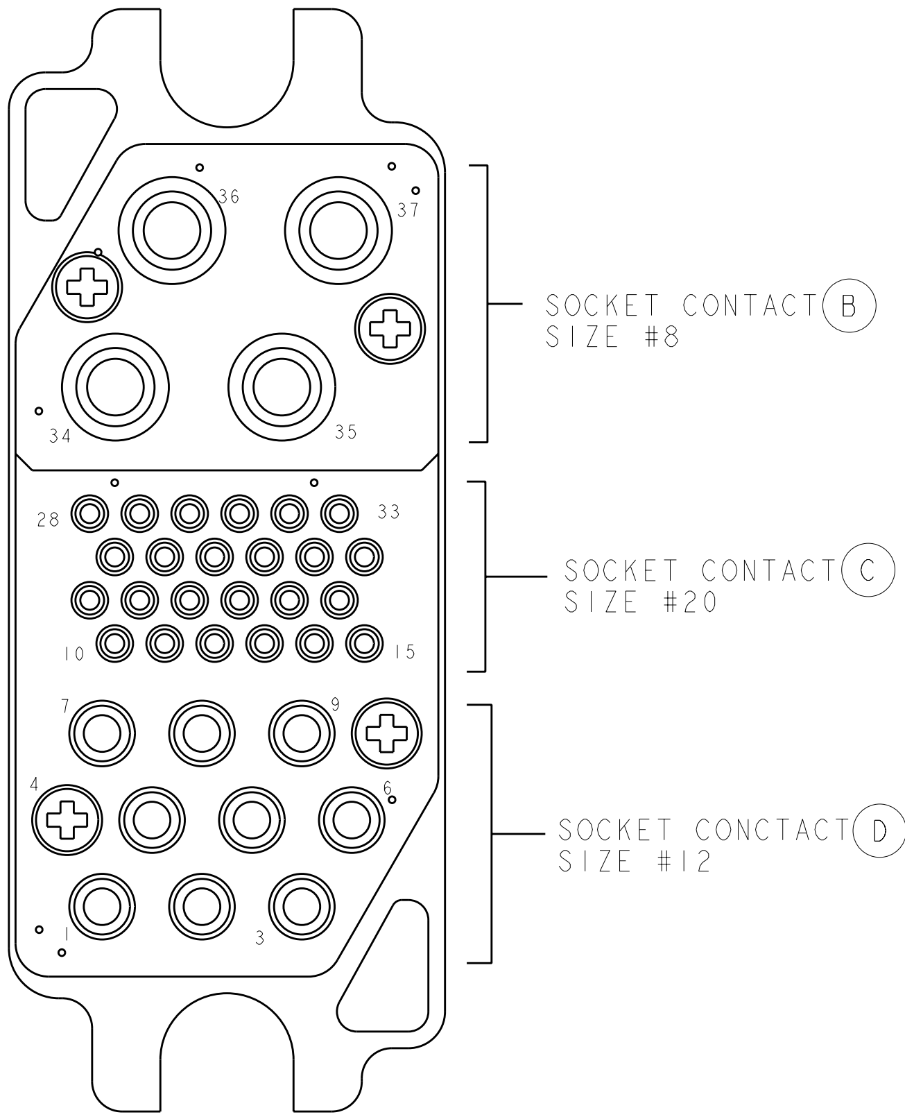
REAR VIEW
