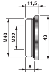
Dimensional drawing
