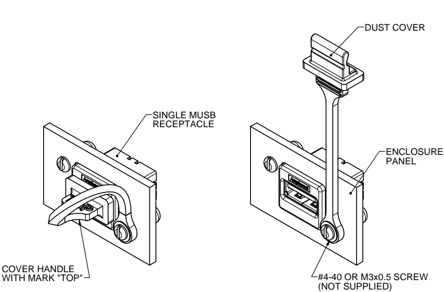
SINGLE MUSB WITH DUST COVER
