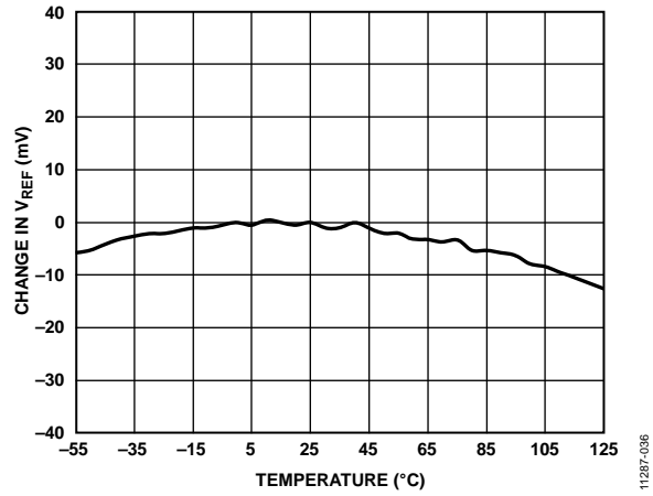
Figure 36. Change in V_{REF} vs. Temperature with Respect to 25°C, P_{IN} = -40 dBm
