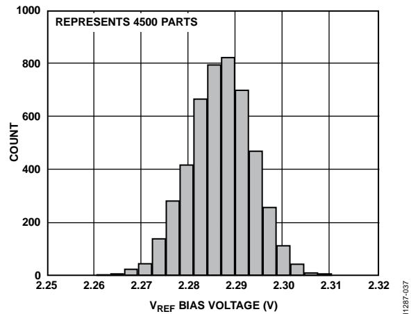
Figure 37. Distribution of V_{REF} at 25°C, No RF Input
