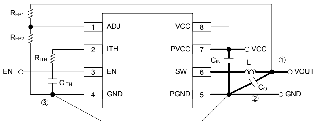
Figure 33. Layout Diagram
