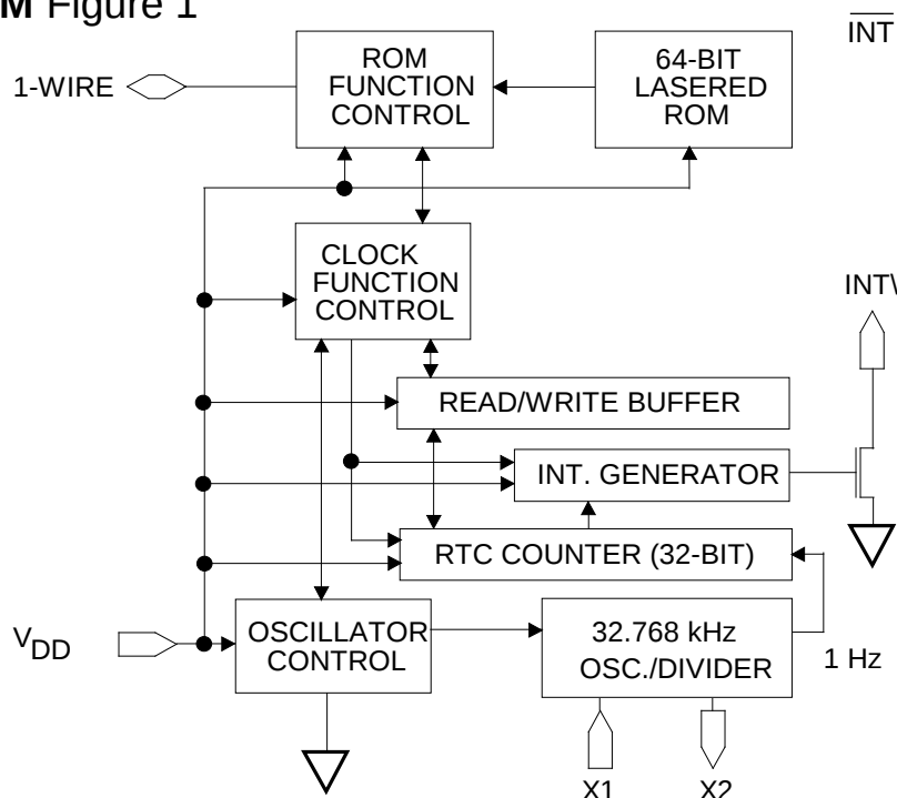
BLOCK DIAGRAM Figure 1
